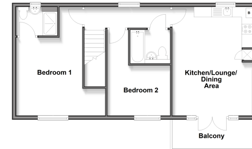
First Floor Approx. 60.7 sq. metres (653.0 sq. feet) (including balcony)
