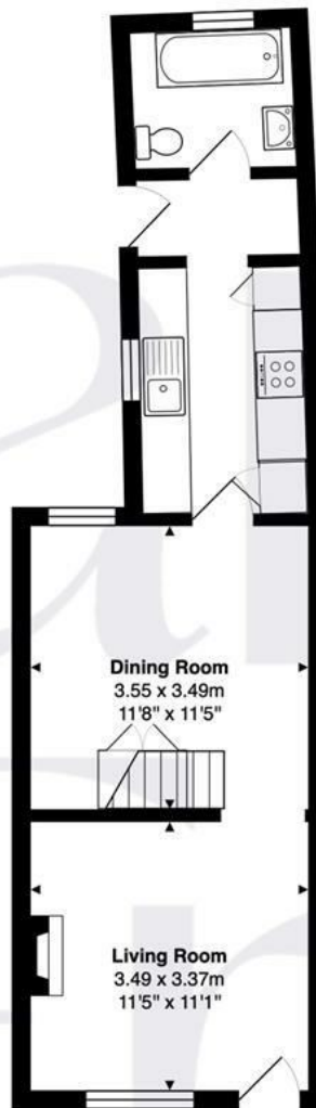
Ground Floor Area: 37.3 m 2 ... 402 ft 2
