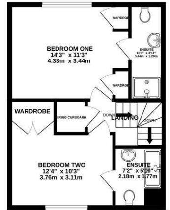
2ND FLOOR 431 sq.ft. (40.0 sq.m.) approx.
