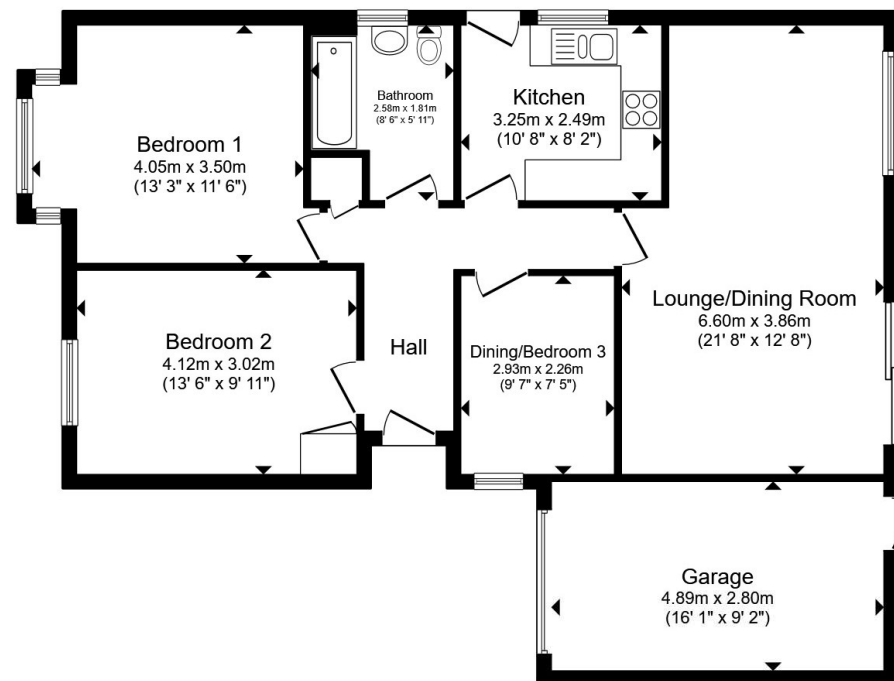
Floor Plan
