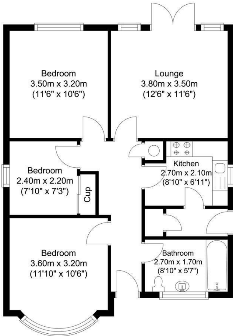
GROUND FLOOR
