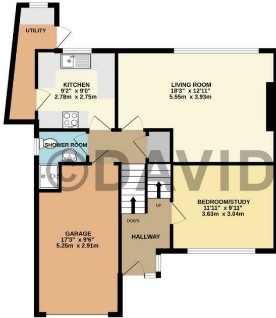
GROUND FLOOR 747 sq.ft. (69.4 sq.m.) approx.
