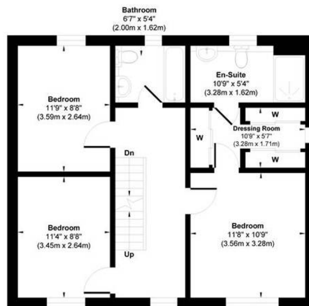
First Floor Approximate Floor Area 636 sq.ft (59.09 sq.m)
