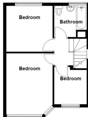
First Floor Approx. 388.6 sq. feet
