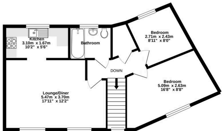
1st Floor 57.5 sq.m. (619 sq.ft.) approx.
