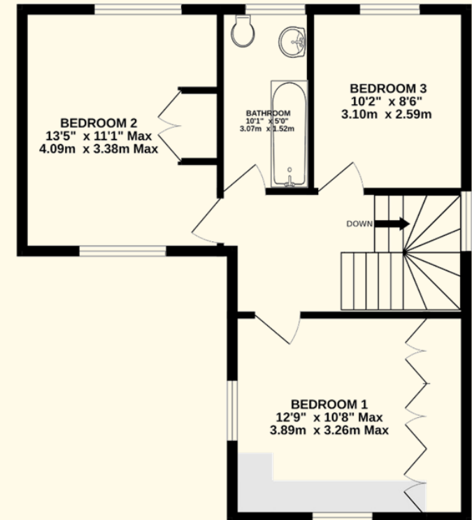
1ST FLOOR 514 sq.ft. (47.7 sq.m.) approx.
