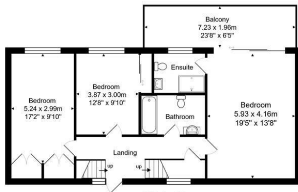
Middle Floor
