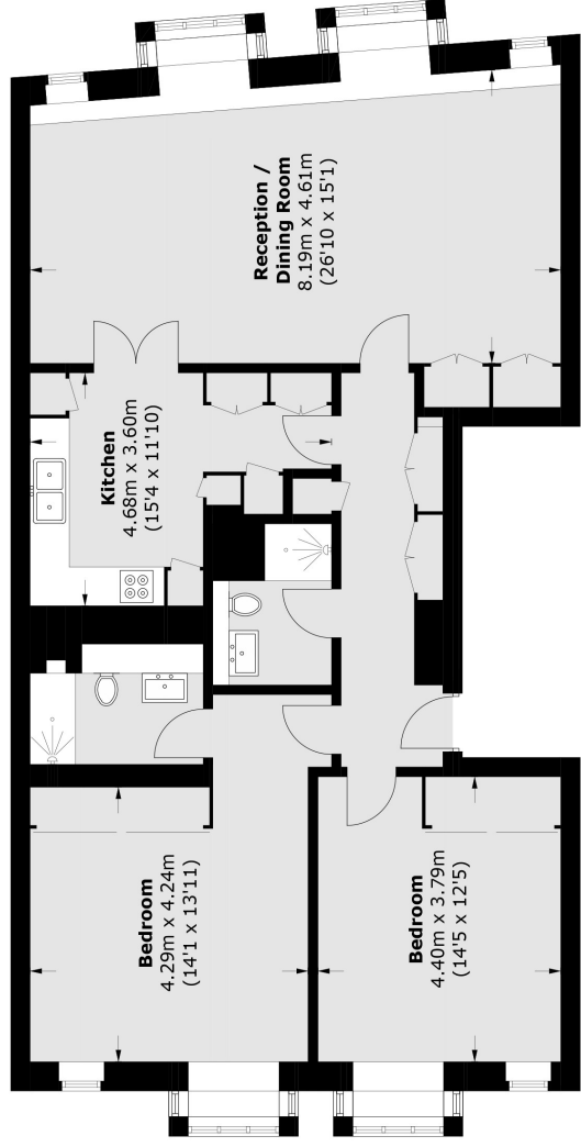
Second Floor
