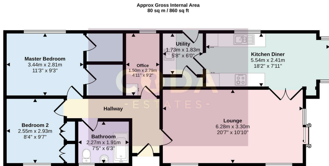
Floorplan
