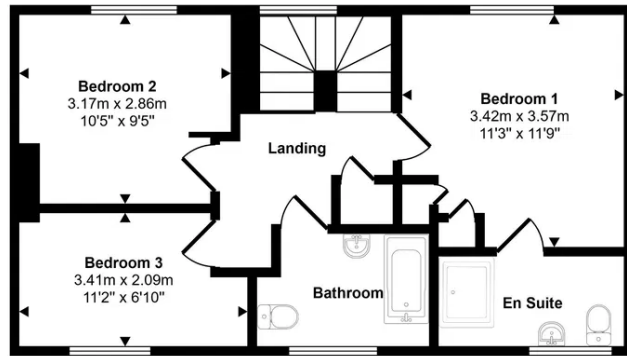
First Floor Approx 47 sq m / 502 sq ft
