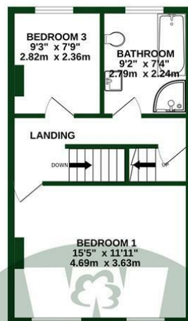
1ST FLOOR 409 sq.ft. (38.0 sq.m.) approx.
