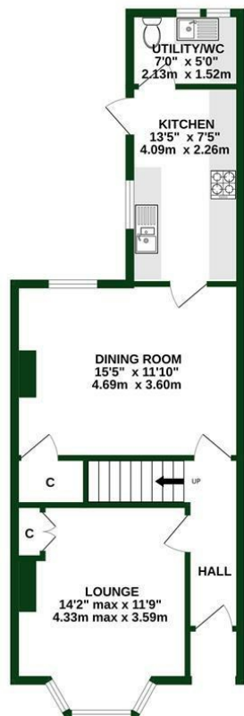
GROUND FLOOR 558 sq.ft. (51.8 sq.m.) approx.
