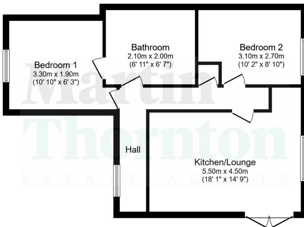
Floor Plan
