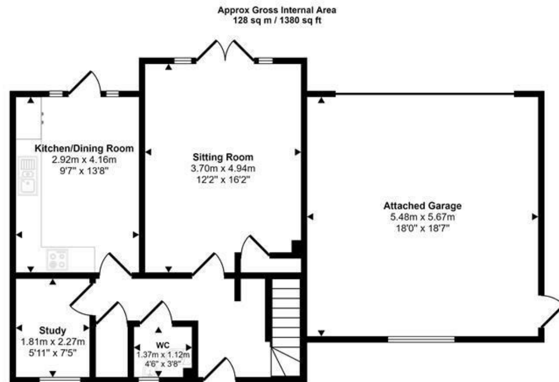
Ground Floor Approx 80 sq m / 857 sq ft
