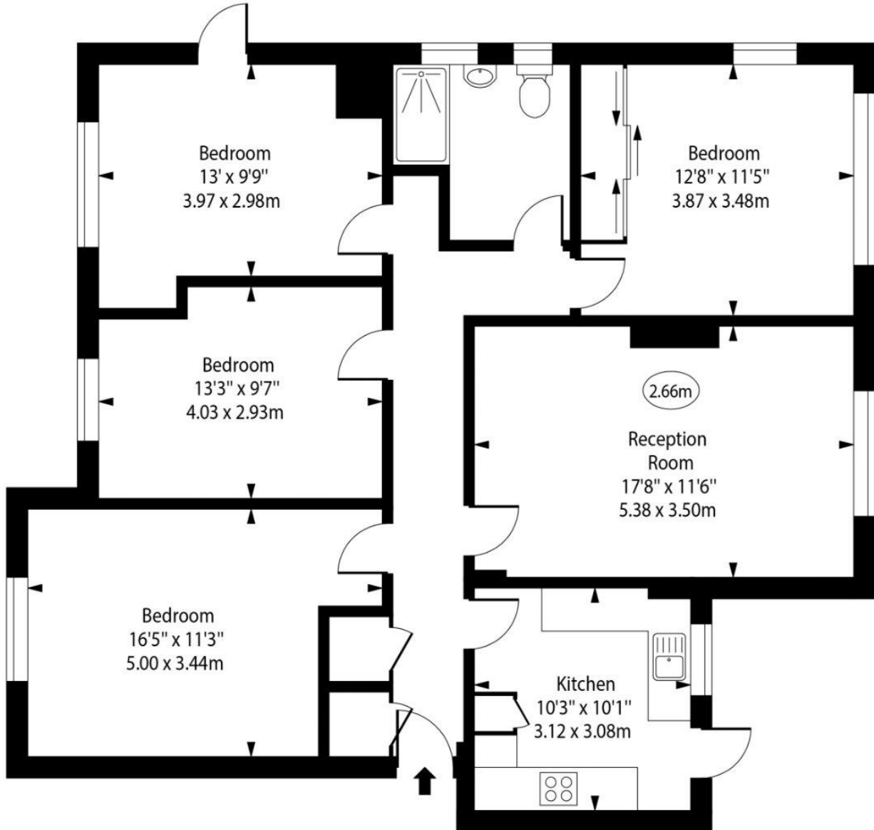
Ground Floor
