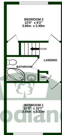
1ST FLOOR 328 sq ft (30.5 sq.m.) approx.
