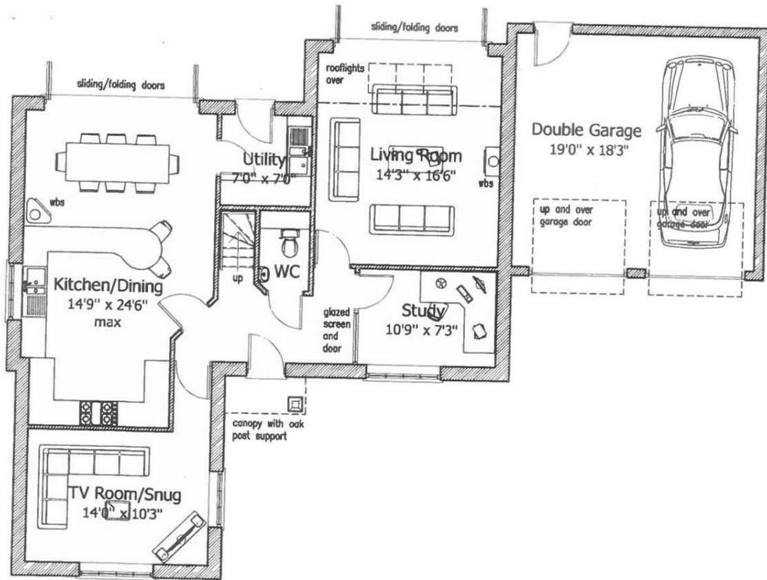
Proposed Indicative Ground Floor Plan - Plot 1 Scale 1:100
