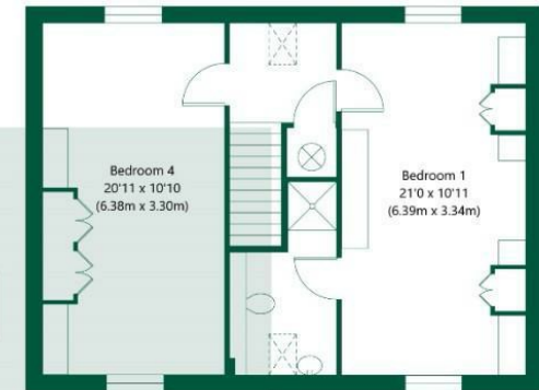
Second Floor GROSS INTERNAL FLOOR AREA APPROX. 602 SQ FT / 55.94 SQ M
