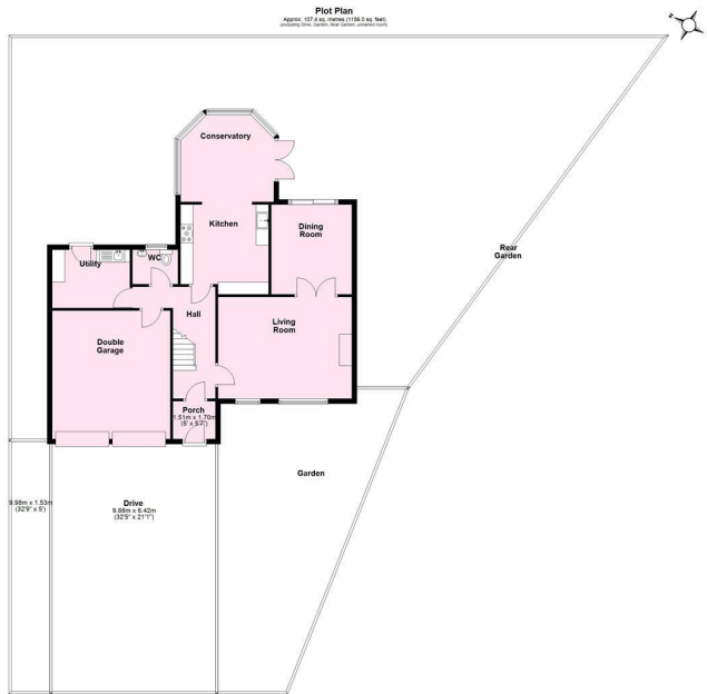
Total area: approx. 107.4 sq. metres (1156.0 sq. feet) Note: Scale for illustration purposes only. Approximate gross internal floor area. Excluding utility areas and storage. All measurements and details including doors and windows are approximate and should be independently verified. Plans produced using PlanIt.
