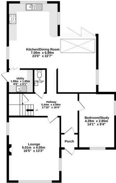
Ground Floor 86.4 sq.m. (930 sq.ft.) approx.
