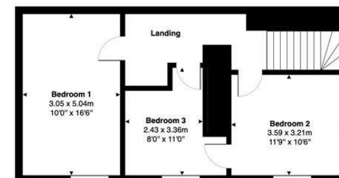
First Floor Area: 51.0 m² ... 549 ft²
