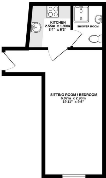
1ST FLOOR 29.0 sq.m. (312 sq.ft.) approx.
