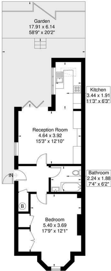
Birkbeck Road Approximate Gross Internal Area = 59.1 sq m / 636 sq ft
