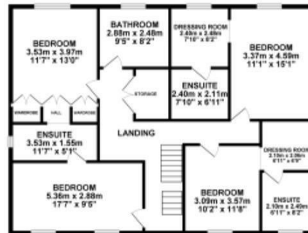
1ST FLOOR 111.23 sq. m. (1197.28 sq. ft.)
