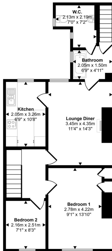
Floorplan
