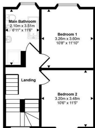
First Floor Approx 41 sq m / 437 sq ft
