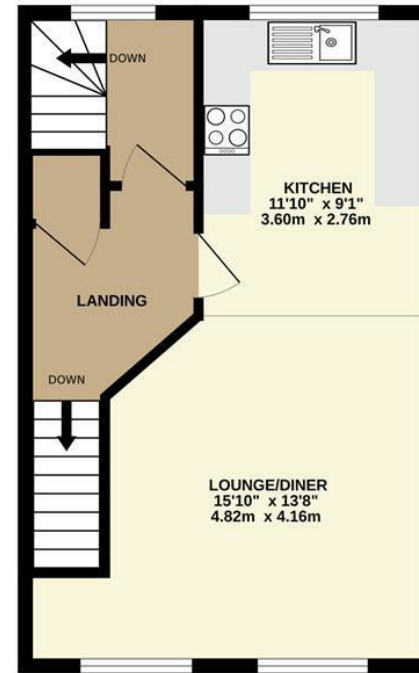
1ST FLOOR 402 sq.ft. (37.4 sq.m.) approx.
