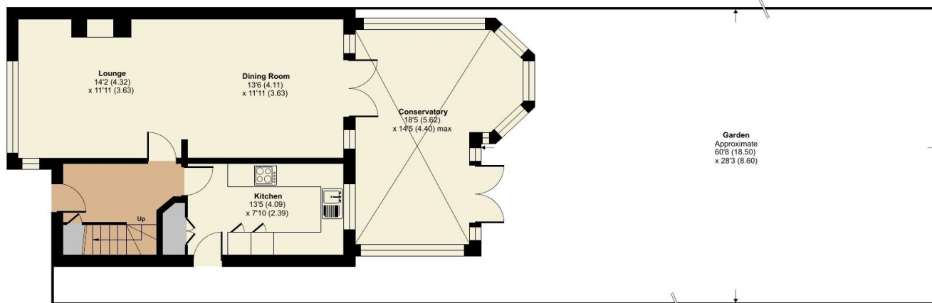
GROUND FLOOR
