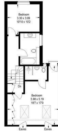
Top Floor
