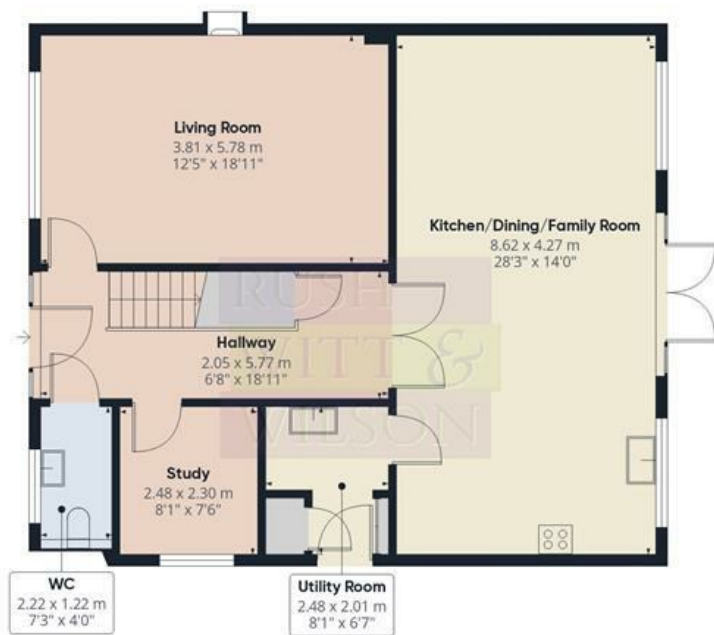
Floor 0 Building 1
