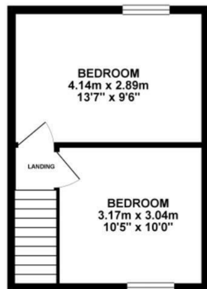
1ST FLOOR 24.54 sq. m. ( 264.11 sq. ft. )
