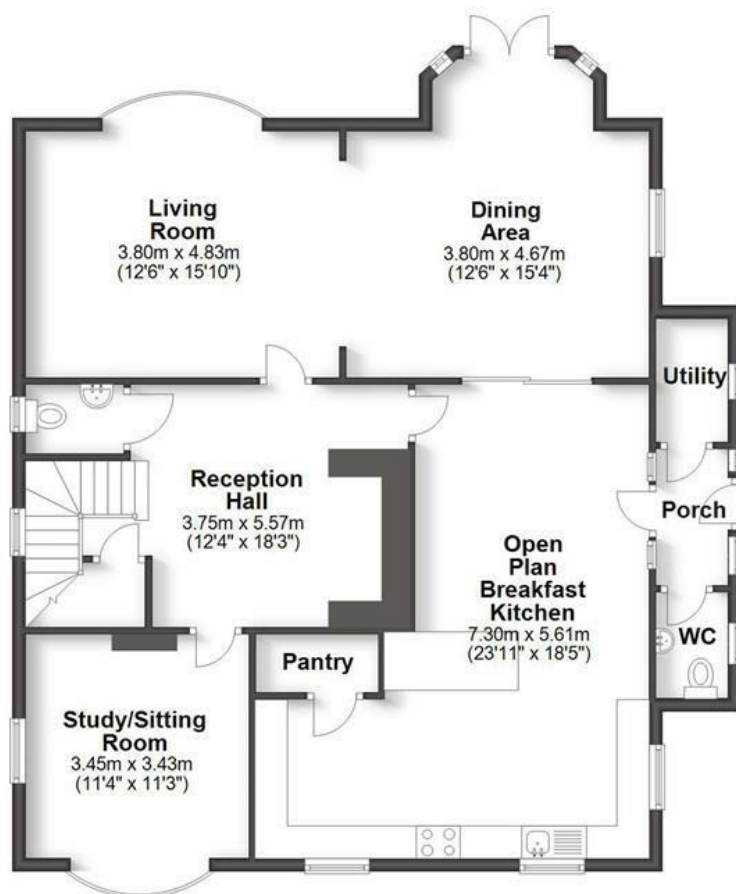
Ground Floor
