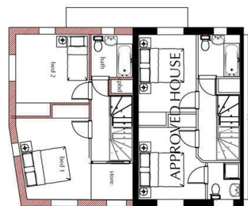
FLOOR LAYOUTS 1:100
