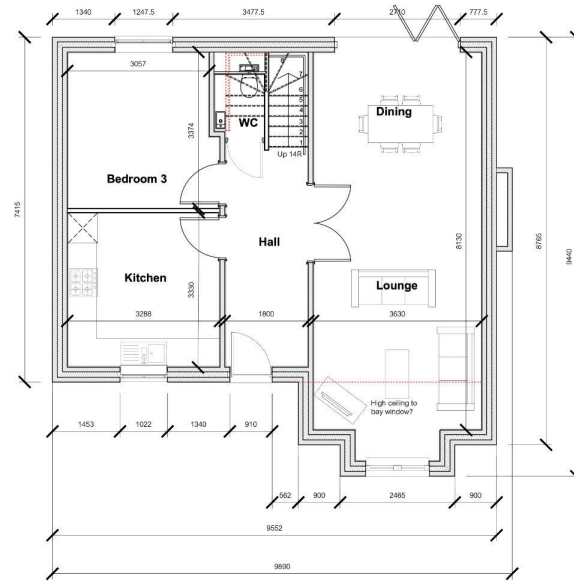
Ground Floor Plan Scale 1:50
