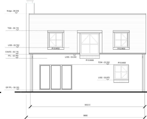
Rear Elevation AA Scale 1:50
