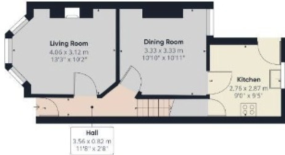
Floor 0 Building 1
