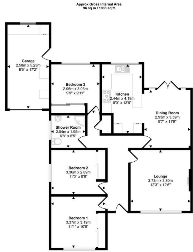
Floorplan
