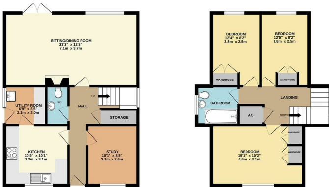
GROUND FLOOR 635 sq. ft. (59.0 sq.m.) approx.
