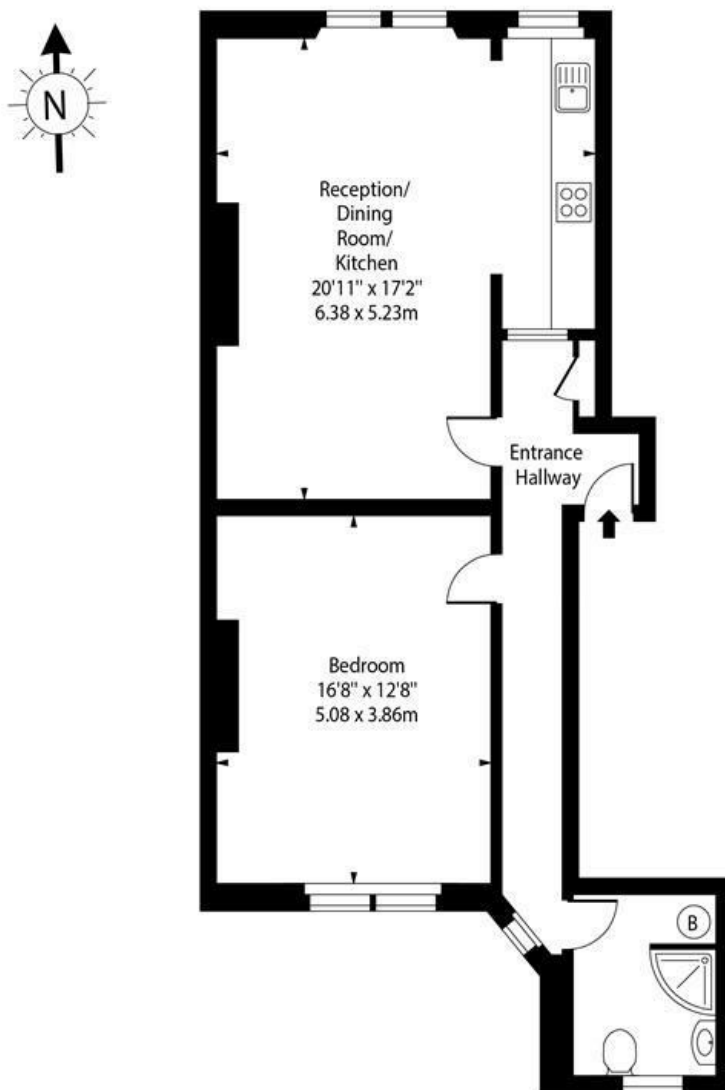
Second Floor
