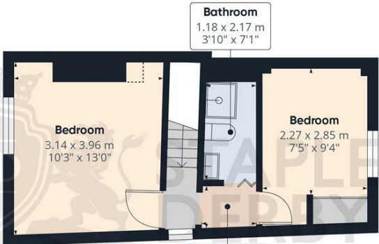
Floor 0 Building 1
