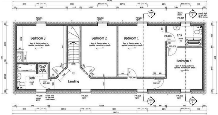
First Floor Plan Scale 1:50
