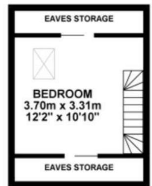
2ND FLOOR 17.92 sq. m. ( 192.91 sq. ft. )
