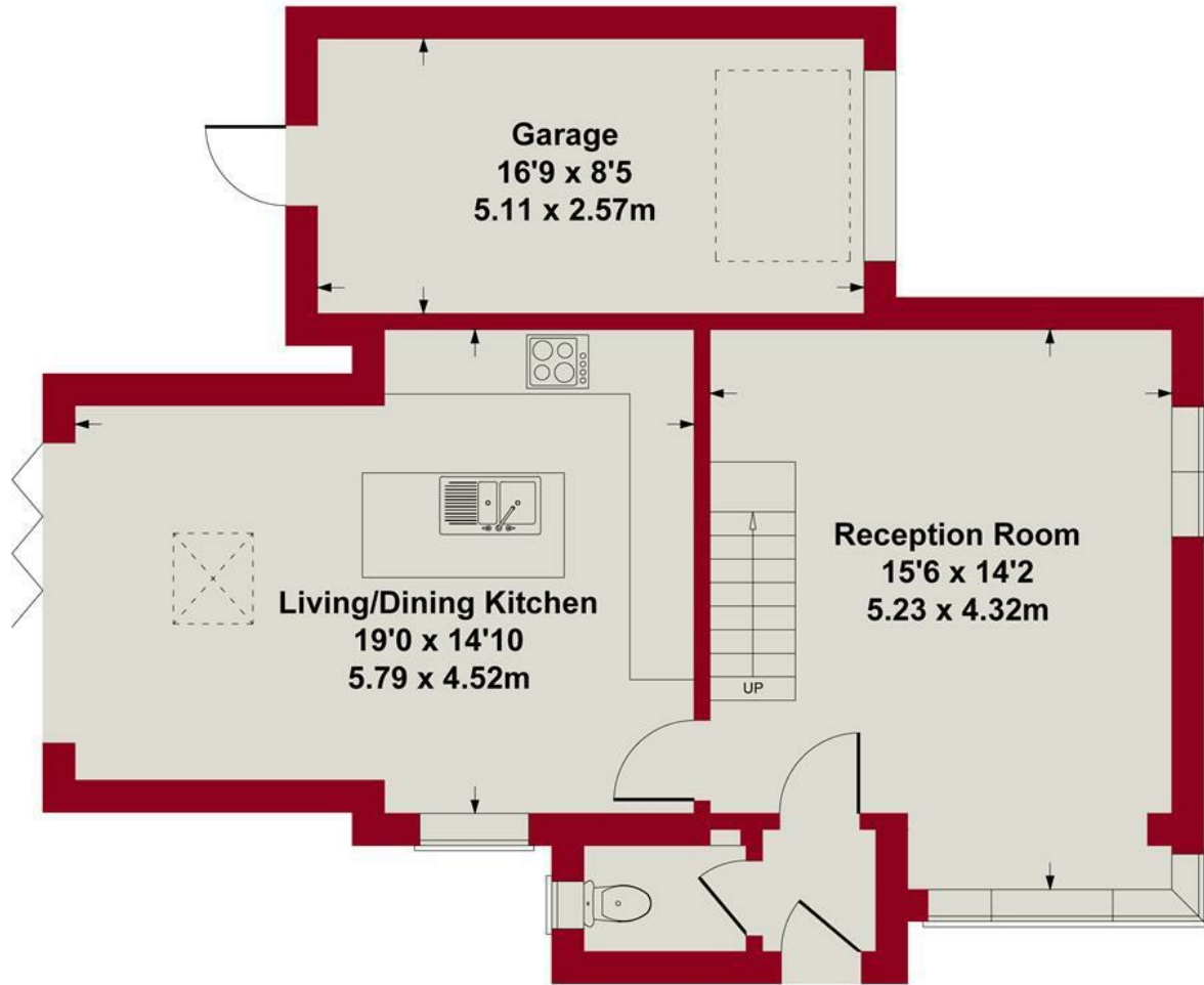
GROUND FLOOR
