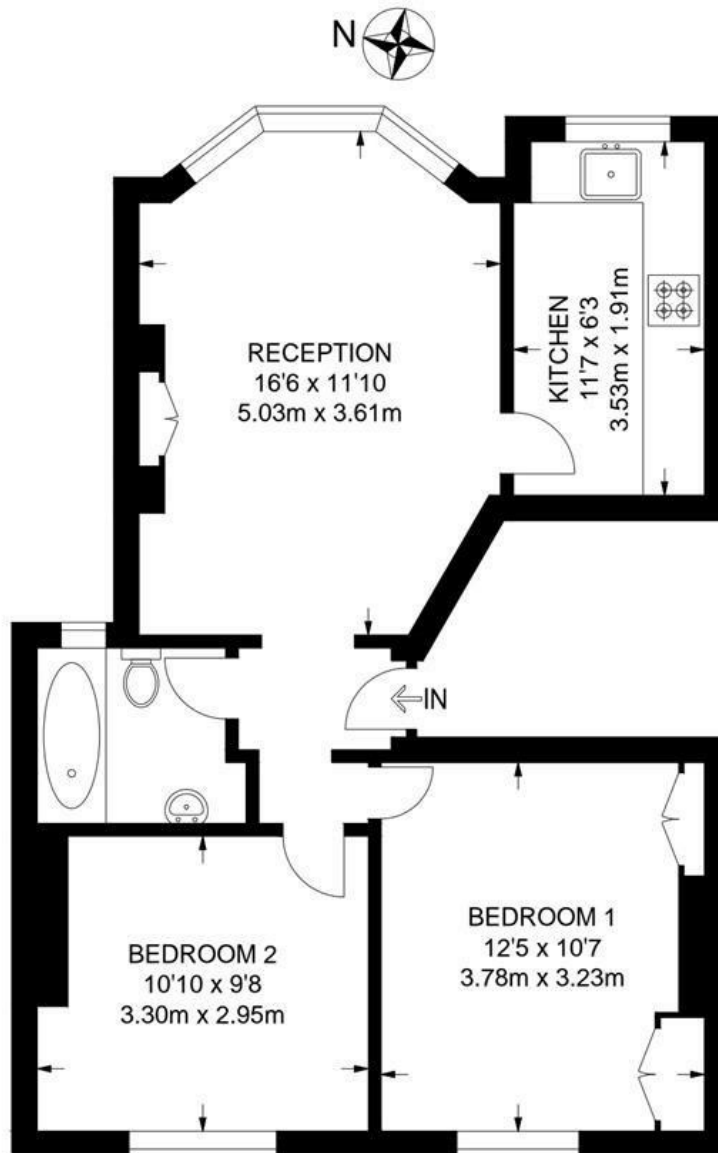
FIRST FLOOR
