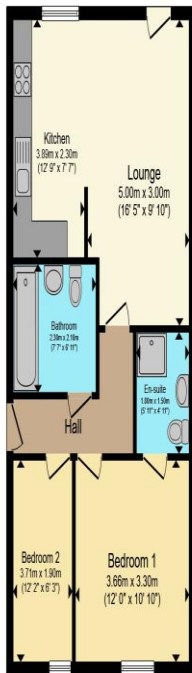
Floor Plan
