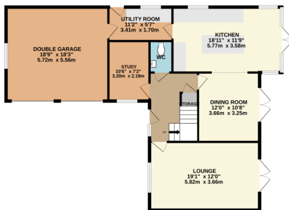
GROUND FLOOR 1229 sq.ft. (224.1 sq.m.) approx.
