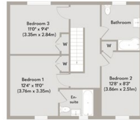
First Floor Approximate Floor Area 599 sq. ft (55.65 sq. m)
