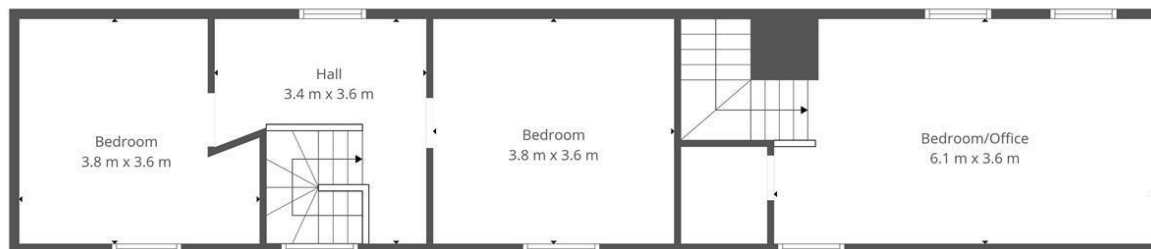
1st Floor
